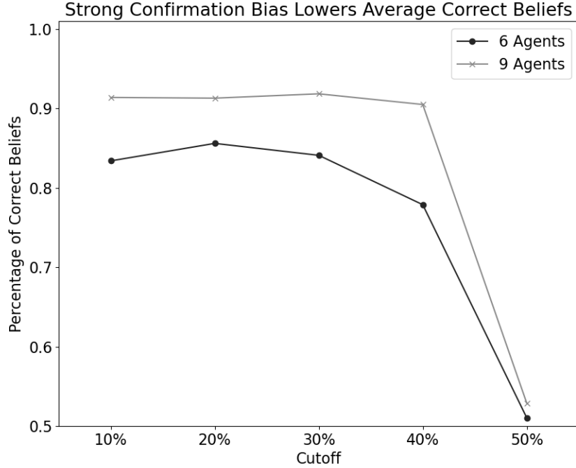
Figure 7: Average correct beliefs under strong confirmation bias. This figure shows results for ER random networks of size 6 and 9, with the probability of connection between any two nodes, b = .5 . Qualitative results are robust across parameter values. \epsilon = .001 , n = 1000
