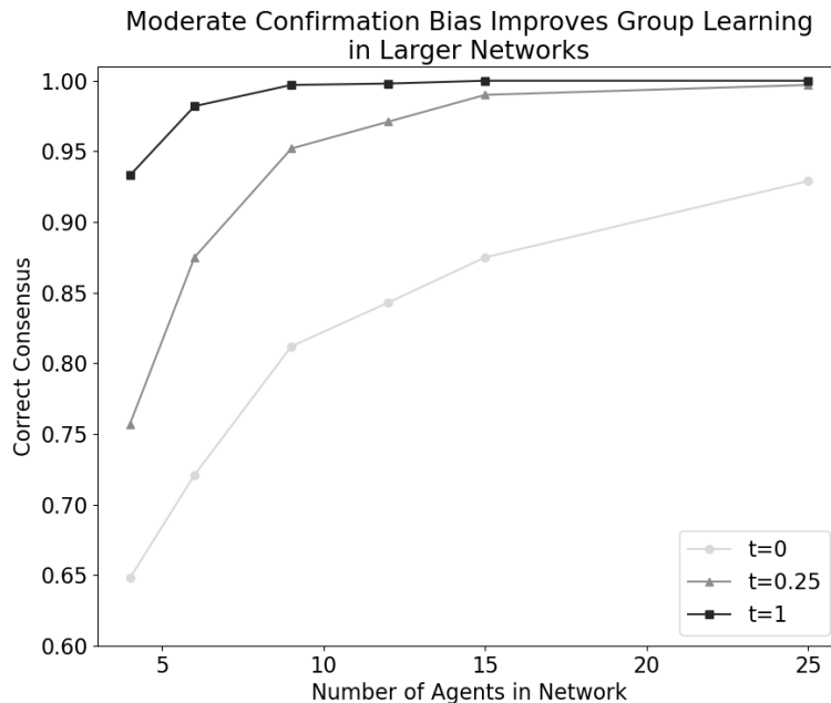
Figure 3: When agents use moderate levels of confirmation bias, groups tend to reach accurate consensus more often. This figure shows results for moderate sized ER random networks with the probability of connection between any two nodes, b = .5 . Qualitative results are robust across parameter values. \epsilon = .001 , n = 1000
