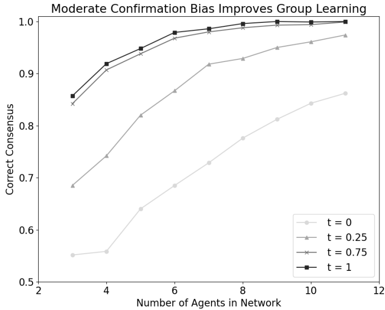
Figure 2: When agents use moderate levels of confirmation bias, groups tend to reach accurate consensus more often. This figure shows results for small wheel networks. Qualitative results are robust across parameter values. \epsilon = .001 , n = 1000
