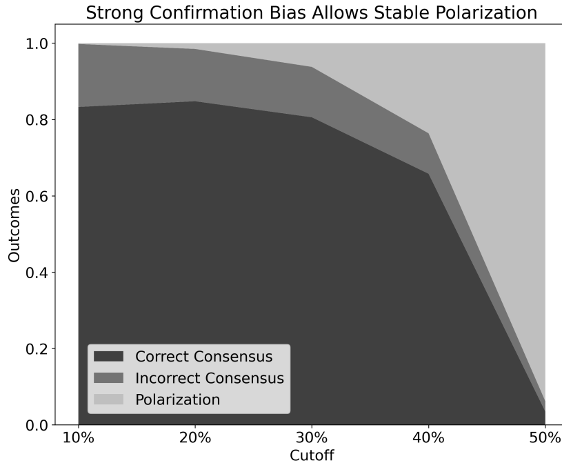
Figure 6: Strong confirmation bias leads to polarization. This figure shows results for ER random networks with the probability of connection between any two nodes, b = .5 . Qualitative results are robust across parameter values. N = 6 , \epsilon = .001 , n = 1000
