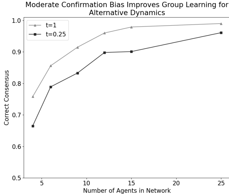
Figure 4: Moderate confirmation bias increases epistemic success under a different operationalization of confirmation bias. This figure shows results for moderate sized ER random networks with the probability of connection between any two nodes, b = .5 . Qualitative results are robust across parameter values. \epsilon = .001 , n = 1000
