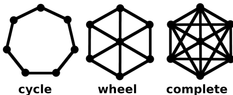
Figure 1: Several network structures
