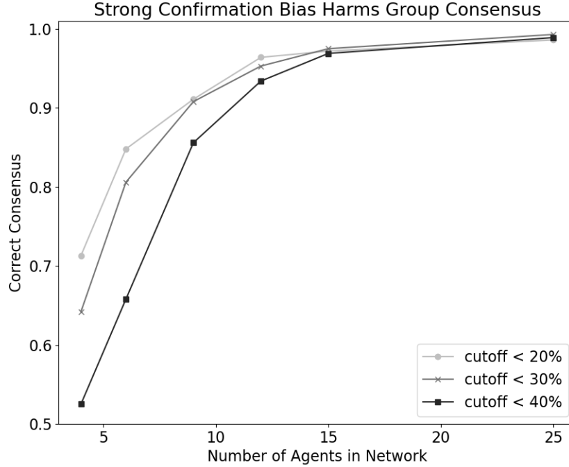
Figure 5: Strong confirmation bias hurts group learning. This figure shows results for moderate sized ER random networks with the probability of connection between any two nodes, b = .5 . Qualitative results are robust across parameter values. \epsilon = .001 , n = 1000
